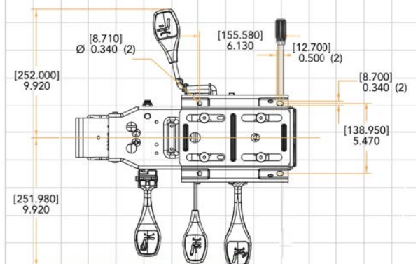
INTEGRATED SEAT SLIDER MOUNTING VIEW TOP PROFILE
