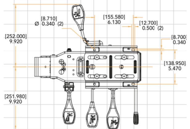
INTEGRATED SEAT SLIDER MOUNTING VIEW TOP PROFILE
